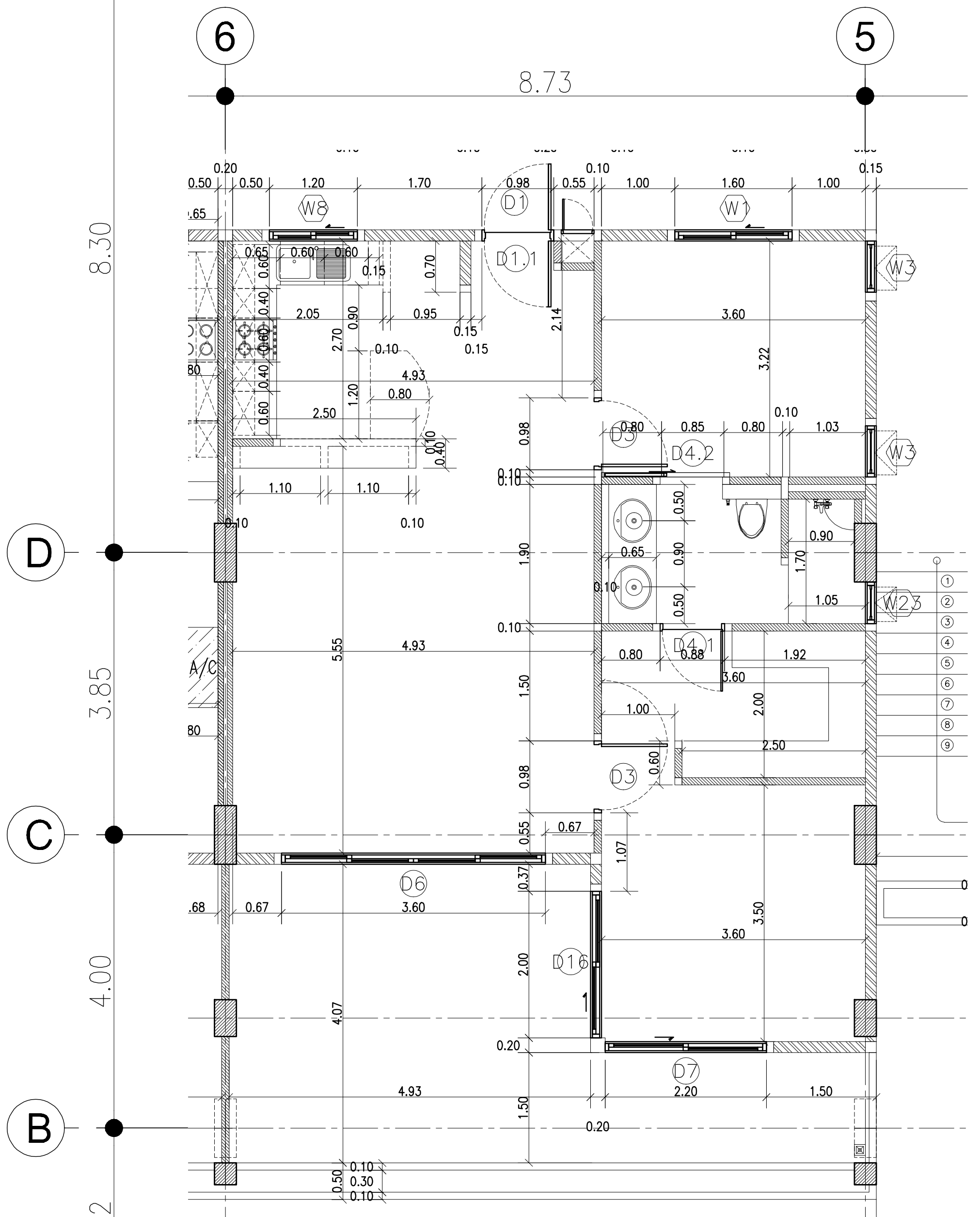
B-24 nd (2 Floor Plan) Scale 1:50
