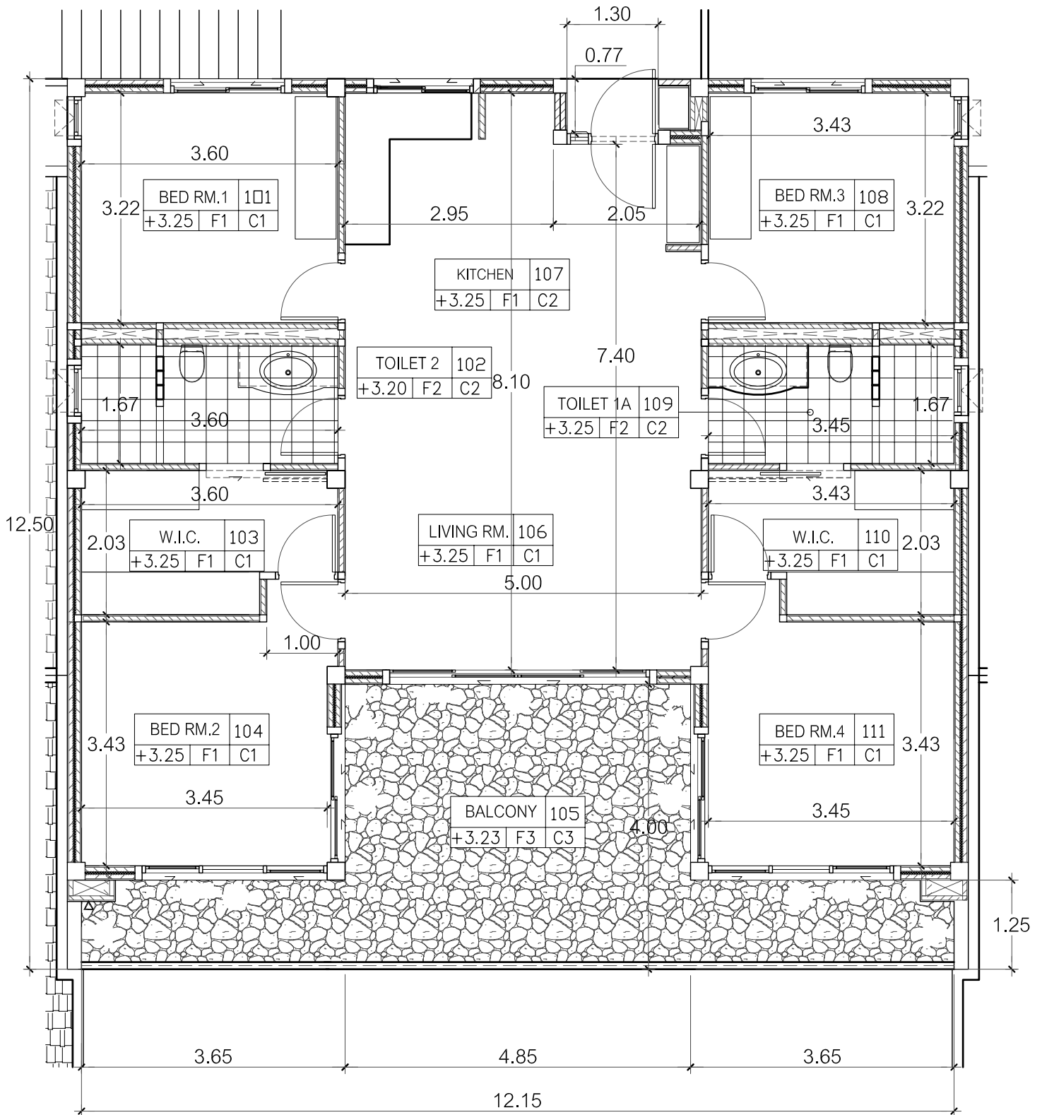
BG 35/36 - B2 SECOND FLOOR PLAN SCALE 1 : 75
